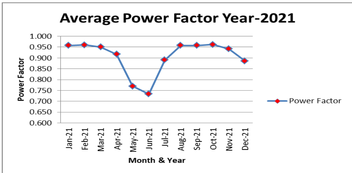
Figure: - Graphical presentation of average power factor of the university Year-2021
